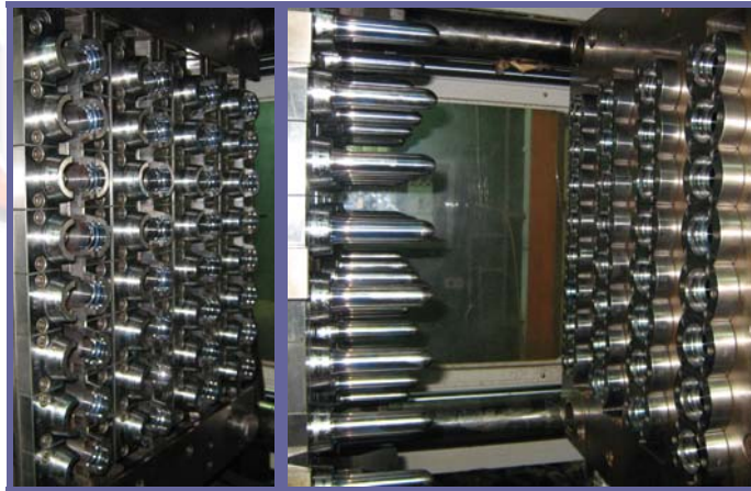
Preform Mold Structure
